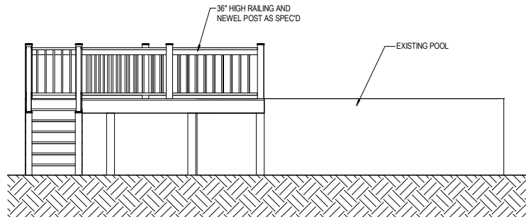
SIDE ELEVATION
