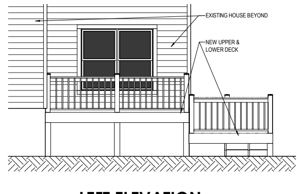
LEFT ELEVATION
